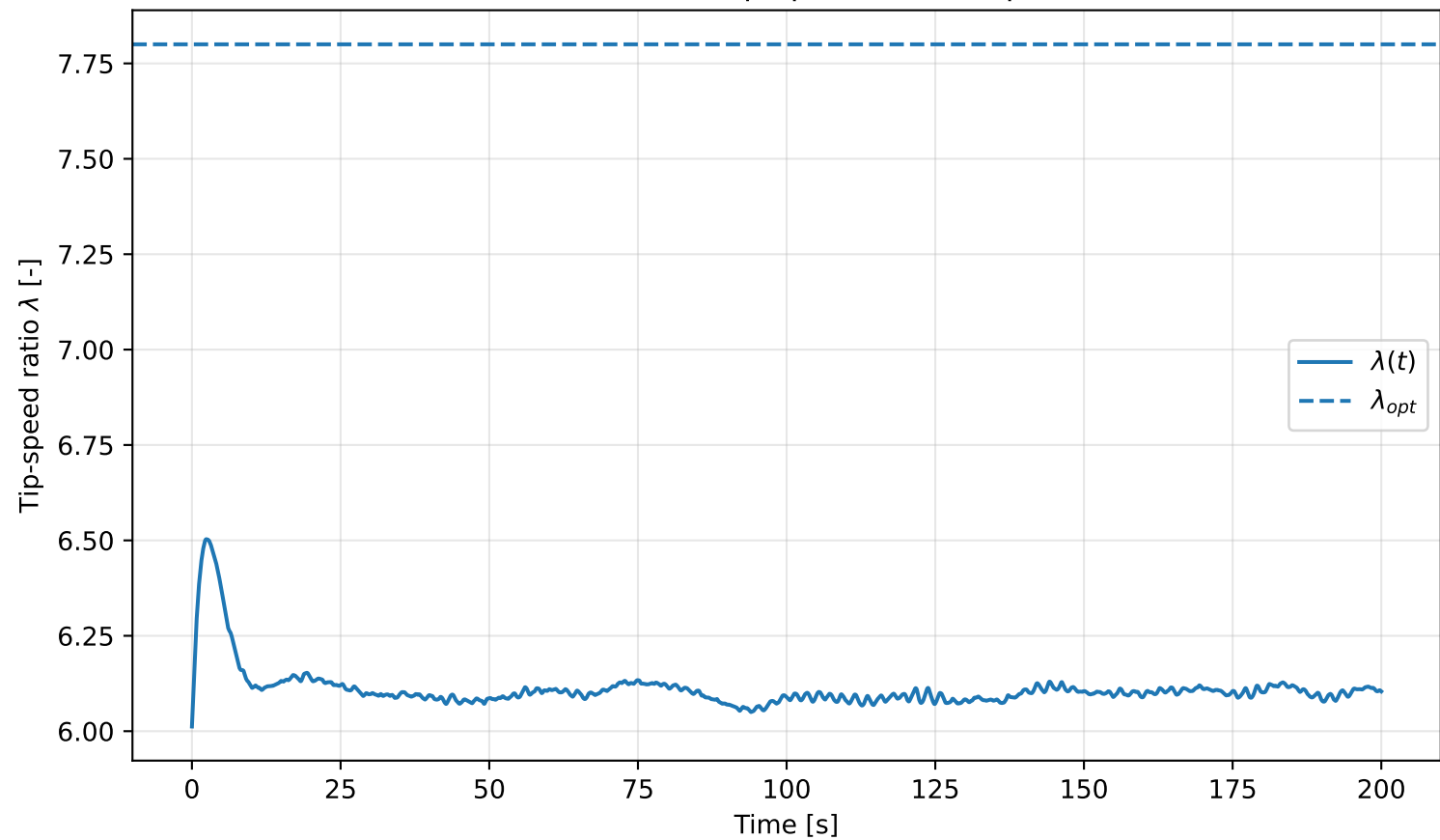
Turbulent wind: tip-speed ratio response
